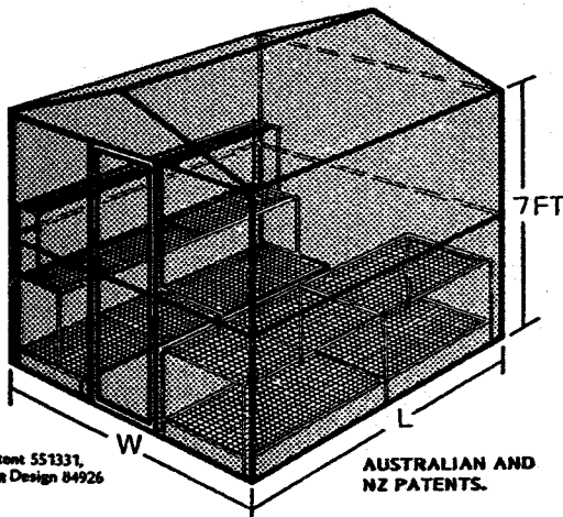
GABLE ROOF SHADEHOUSE KITS ( 2.15m / 7FT WALLS )
